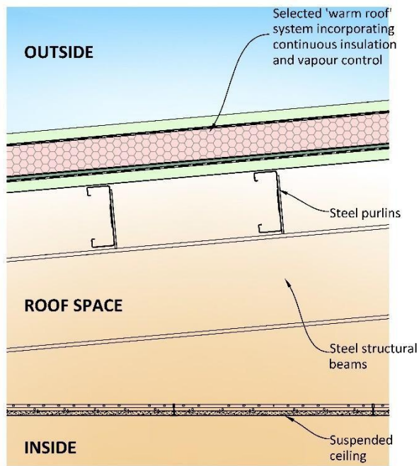
a) Warm roof
