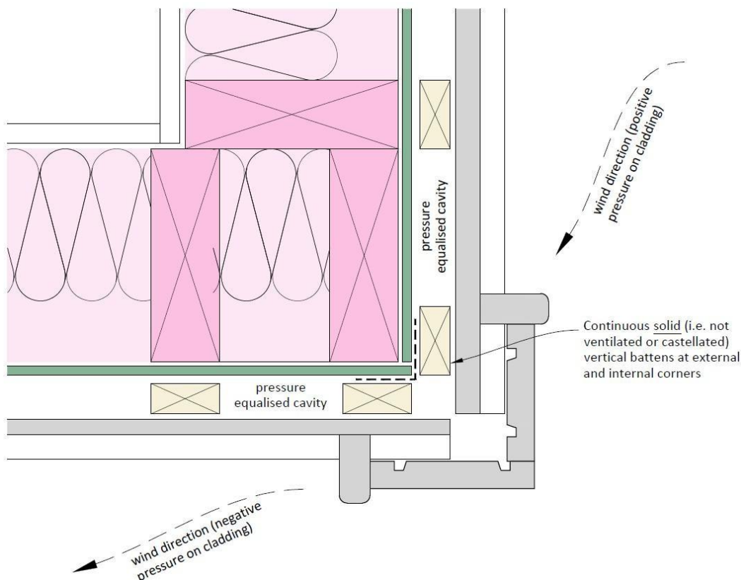
Figure 9-2: Cavity Compartmentalisation at Corner
