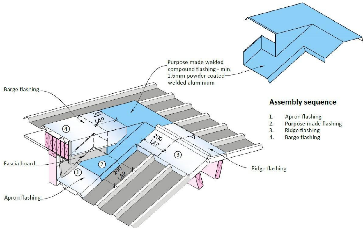
Figure 10-4: Example of 3D Junction – Roof to Barge
