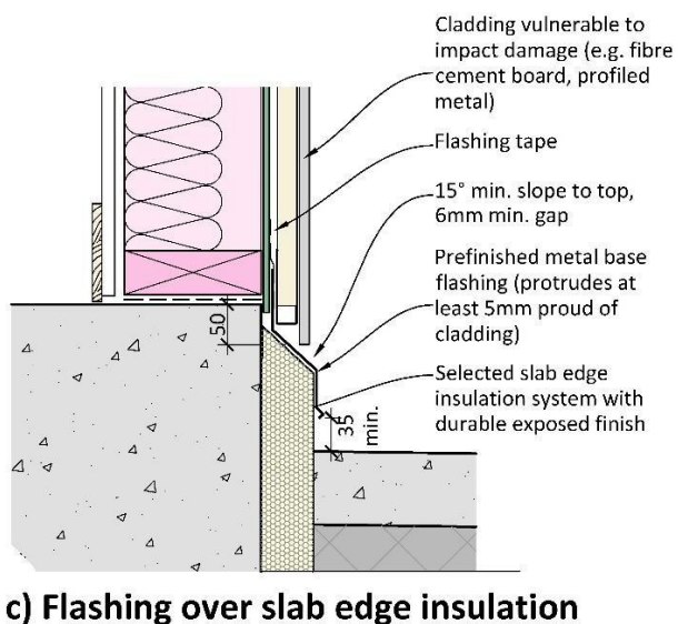
Figure 9-1: Cladding Base Protection Options
