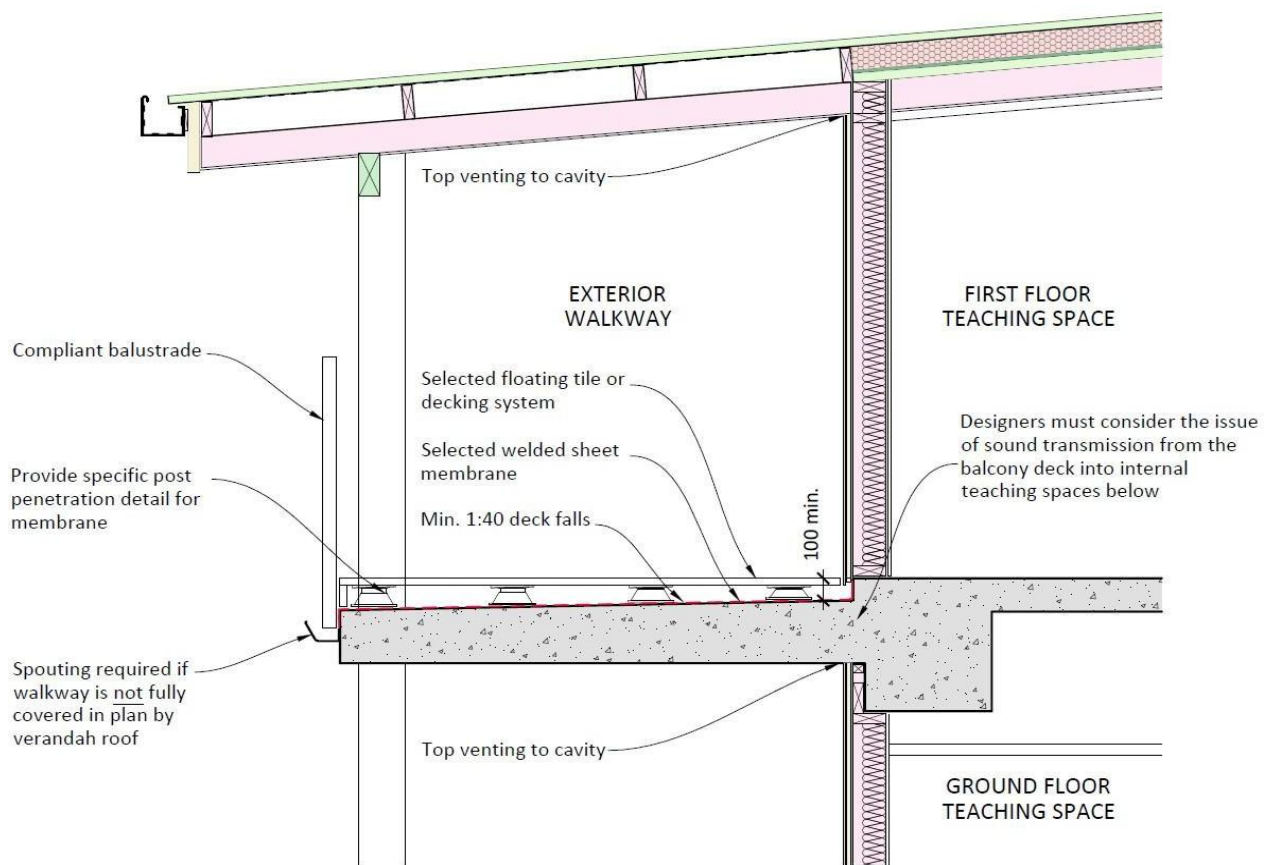
Figure 12-2: Waterproofing to Upper Decks – Non-trafficable Membrane with Floating Deck/ Tiles
