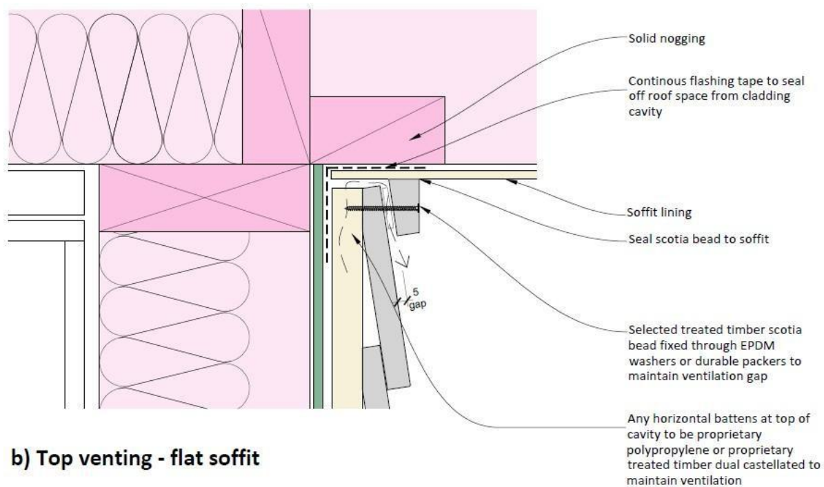
Figure 9-3: Top Venting
