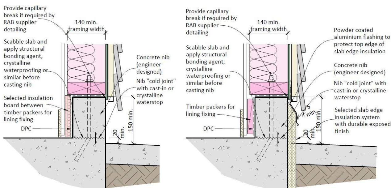
Figure 6-8: Concrete Nib Examples
