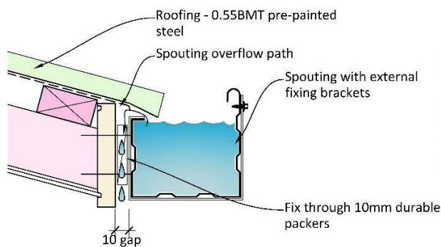
Option 1 - Rear overflow
