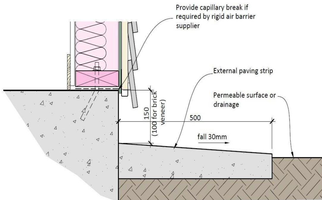
Figure 6-10: External Paving Strip
