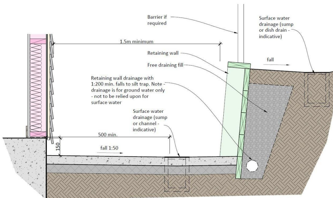
Figure 5-1: Example of Retaining Wall as a Separate Structure
