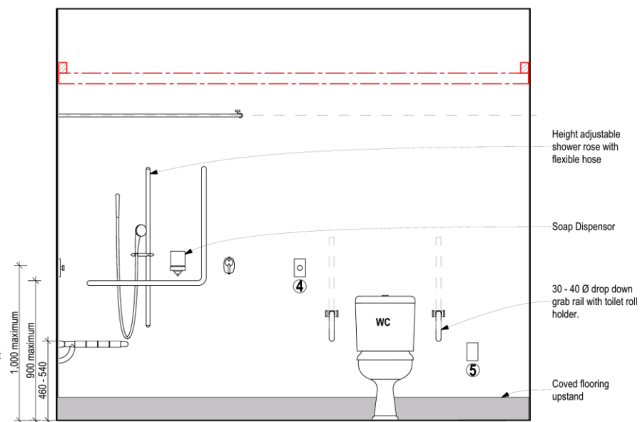
ELEVATION 2 UNIVERSAL BATHROOM
