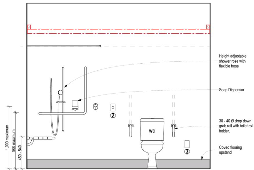
ELEVATION 2 MODIFIED UNIVERSAL BATHROOM
