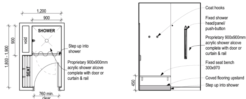
5 SELF-CONTAINED SHOWER WITH SEAT 1:50
