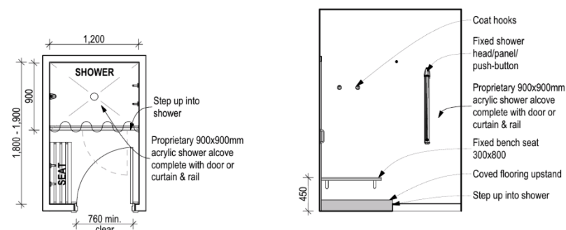
6 SELF-CONTAINED SHOWER WITH SEAT 1:50
