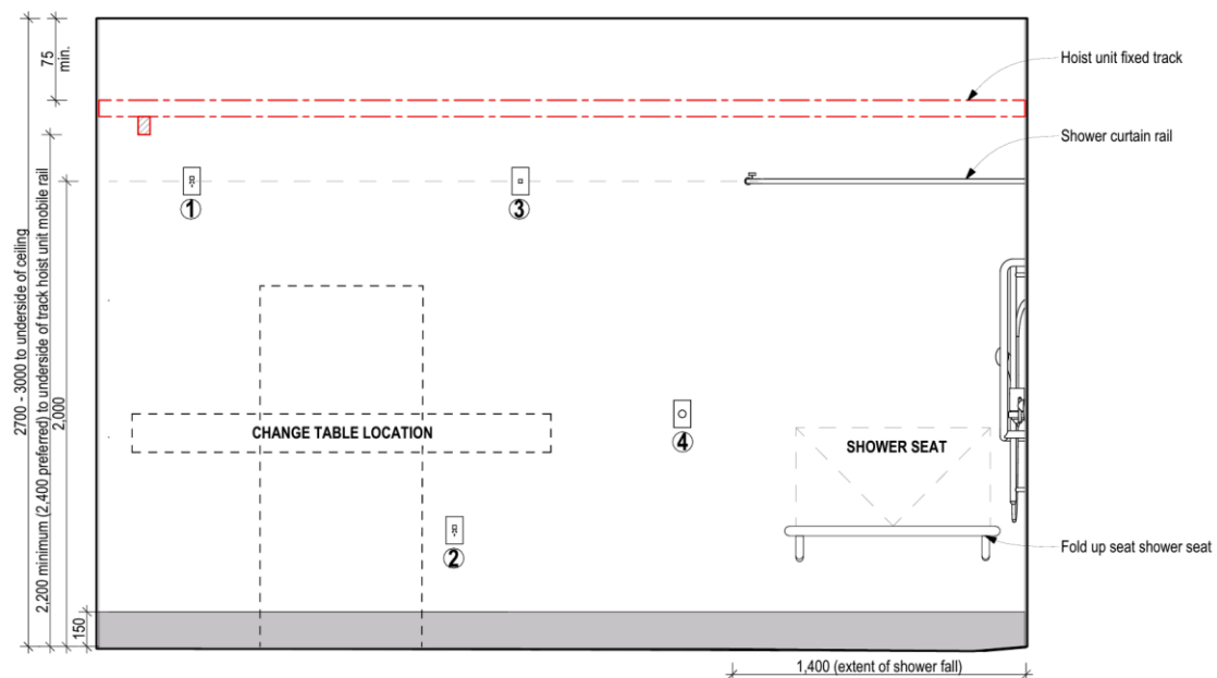
ELEVATION 1 UNIVERSAL BATHROOM
