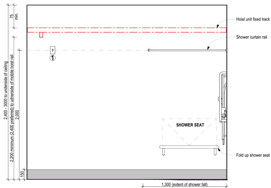
ELEVATION 1 MODIFIED UNIVERSAL BATHROOM
