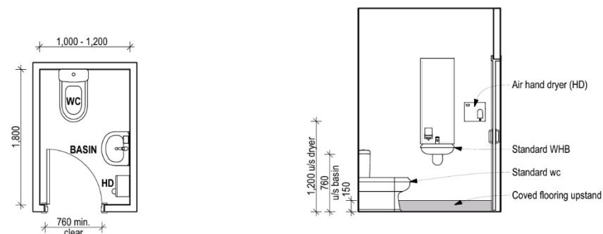
1 STANDARD WC OPTION ONE 1:50
