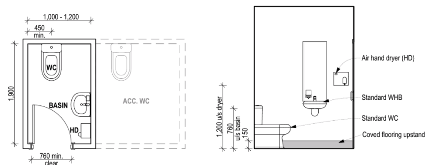
3 STANDARD WC OPTION THREE 1:50
