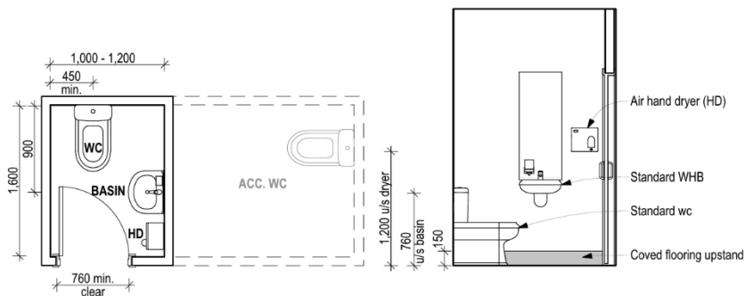
1 STANDARD WC OPTION ONE 1:50
