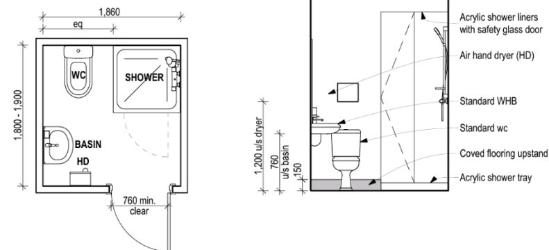
4 STANDARD WC WITH SHOWER 1:50
