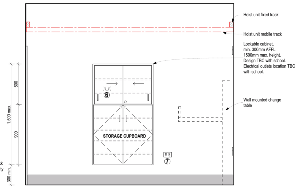
ELEVATION 4 UNIVERSAL BATHROOM
