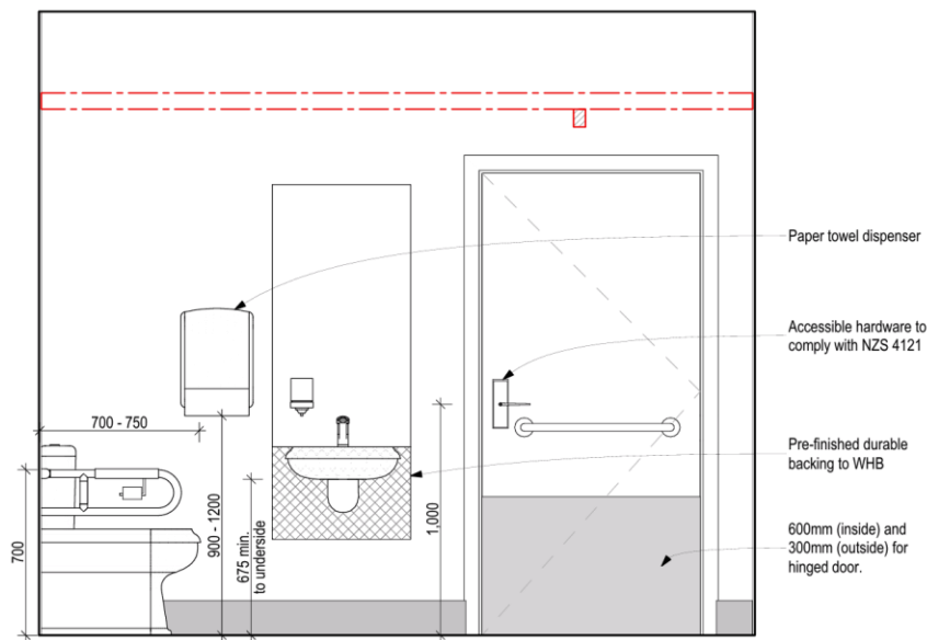
ELEVATION 3 MODIFIED UNIVERSAL BATHROOM
