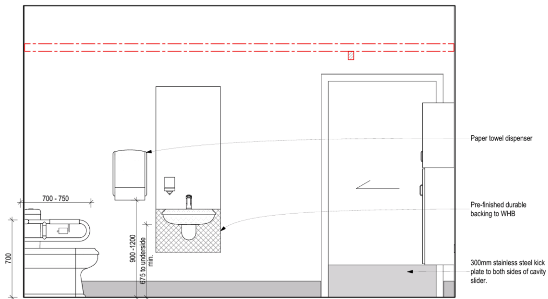
ELEVATION 3 UNIVERSAL BATHROOM
