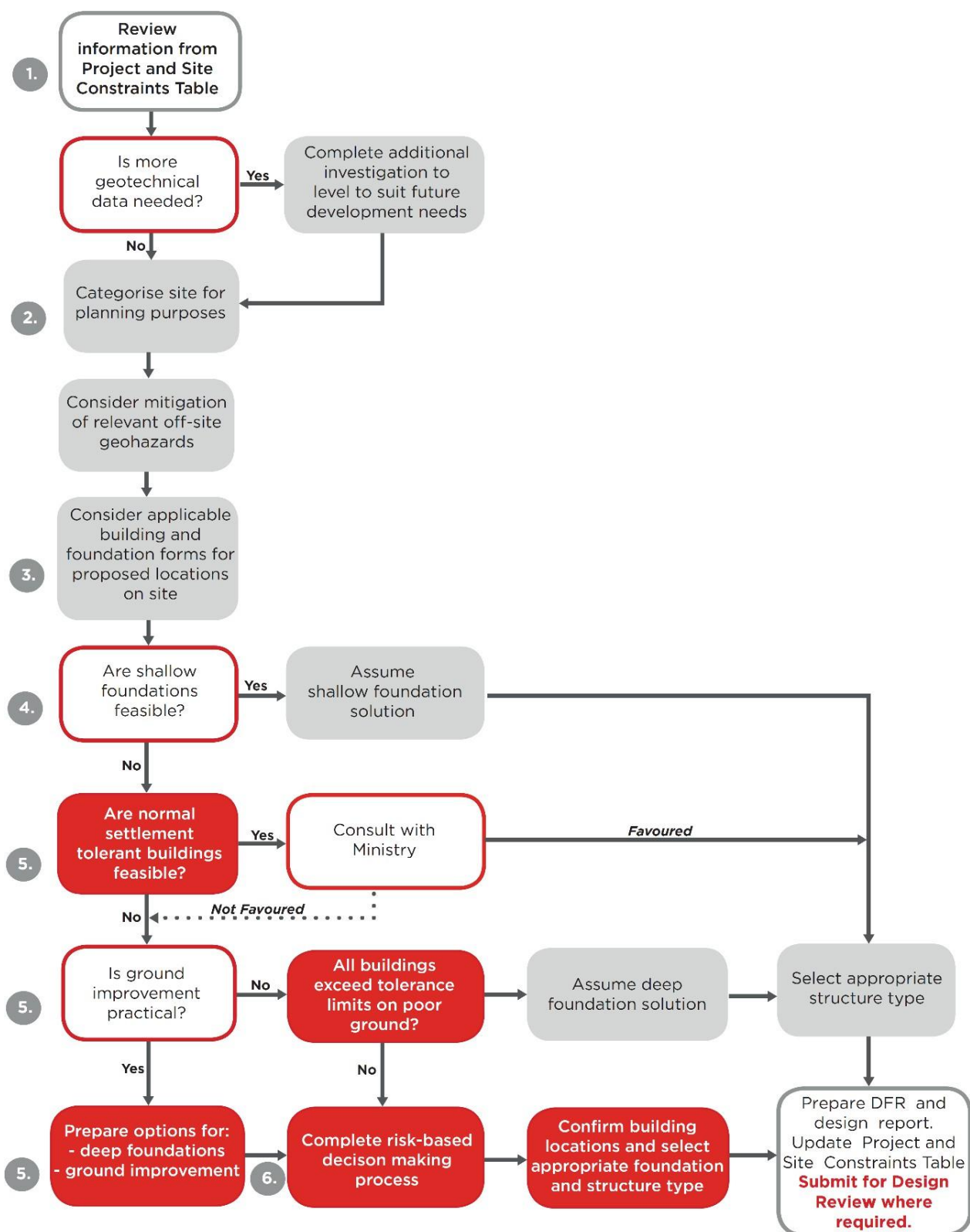
Figure 2.1: Master Planning structural and geotechnical risk assessment
