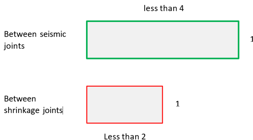
Figure 9.2: Maximum slab panel aspect ratios
