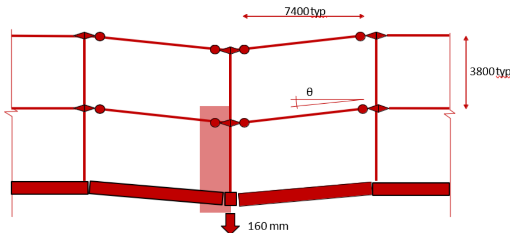
Figure B1: Single Column Frame
