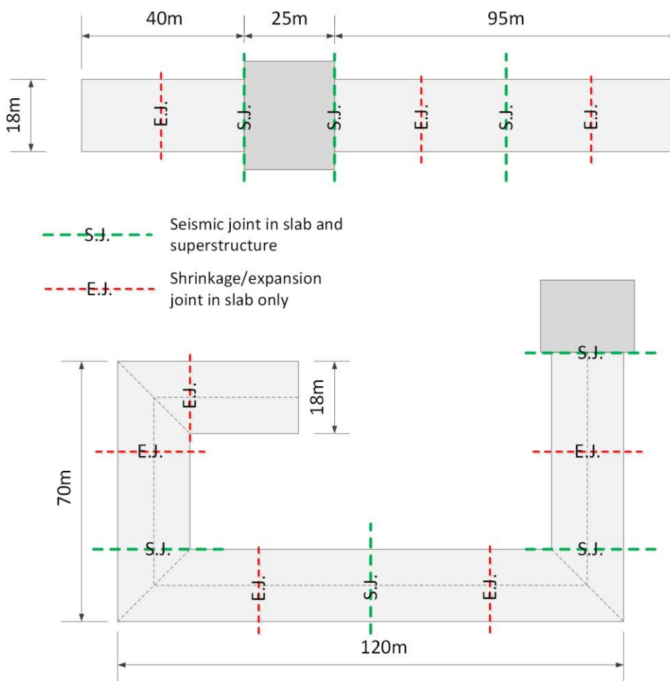
Figure 9.1: Example building plan configurations and joint layouts
