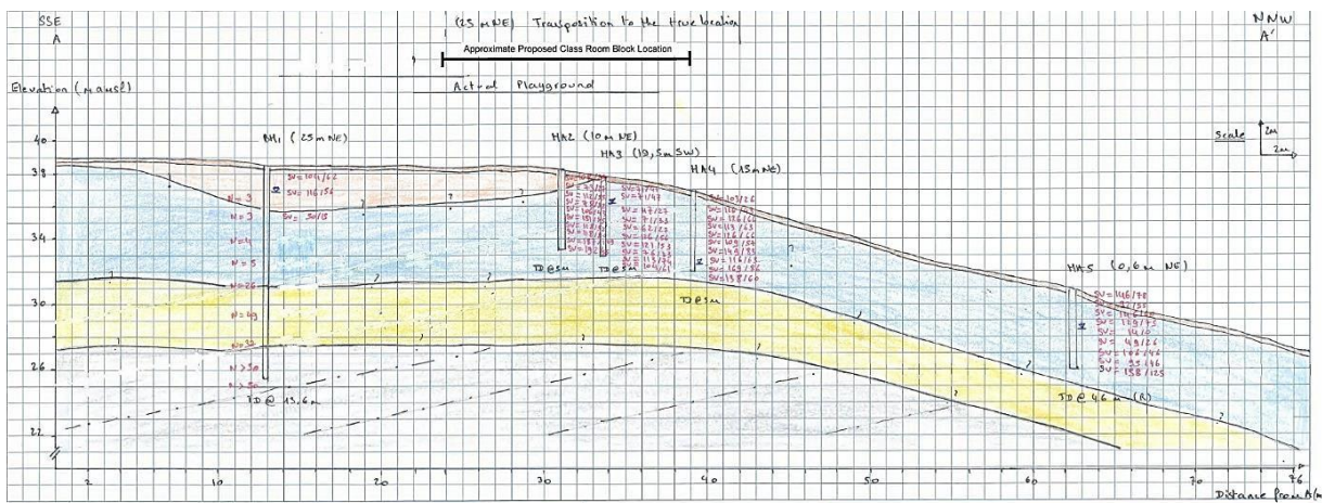
Figure 6.2: Example geotechnical cross section
