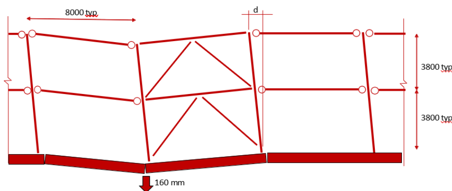
Figure B2: Single Column Frame
