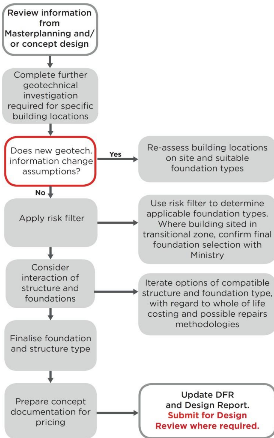
Figure 2.2: Preliminary Design process
