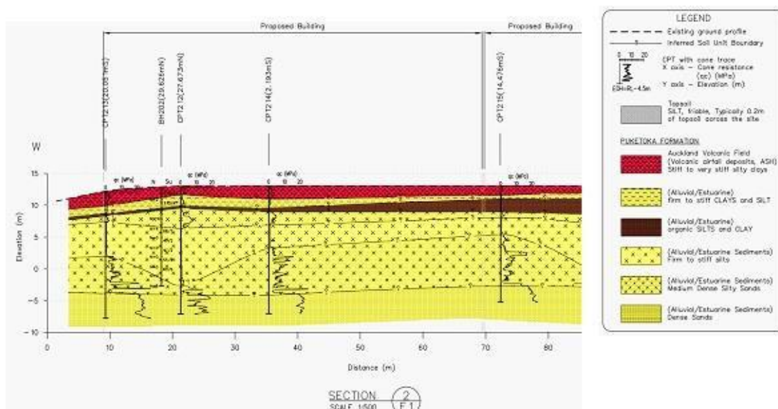
Figure 3.1: Example graphical representation of the site geotechnical mode
