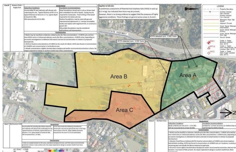
Figure 6.1: Example of a site zonation plan
