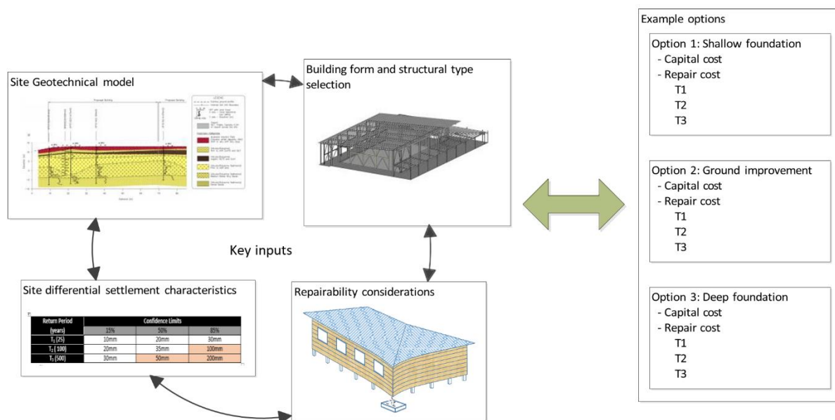
Figure 7.1: Framework for risk-based selection process
