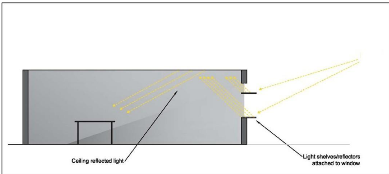
Figure 18: Daylight Reflectors
