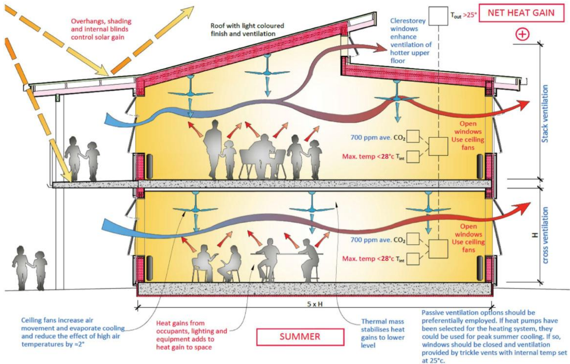
Figure 8: Summer ventilation modes for typical flexible learning spaces
