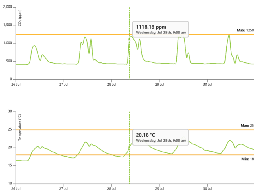
Figure 22: Average CO 2 concentration and temperature levels, in Auckland District over five winter days, between 12am – 12pm in a primary school learning space
