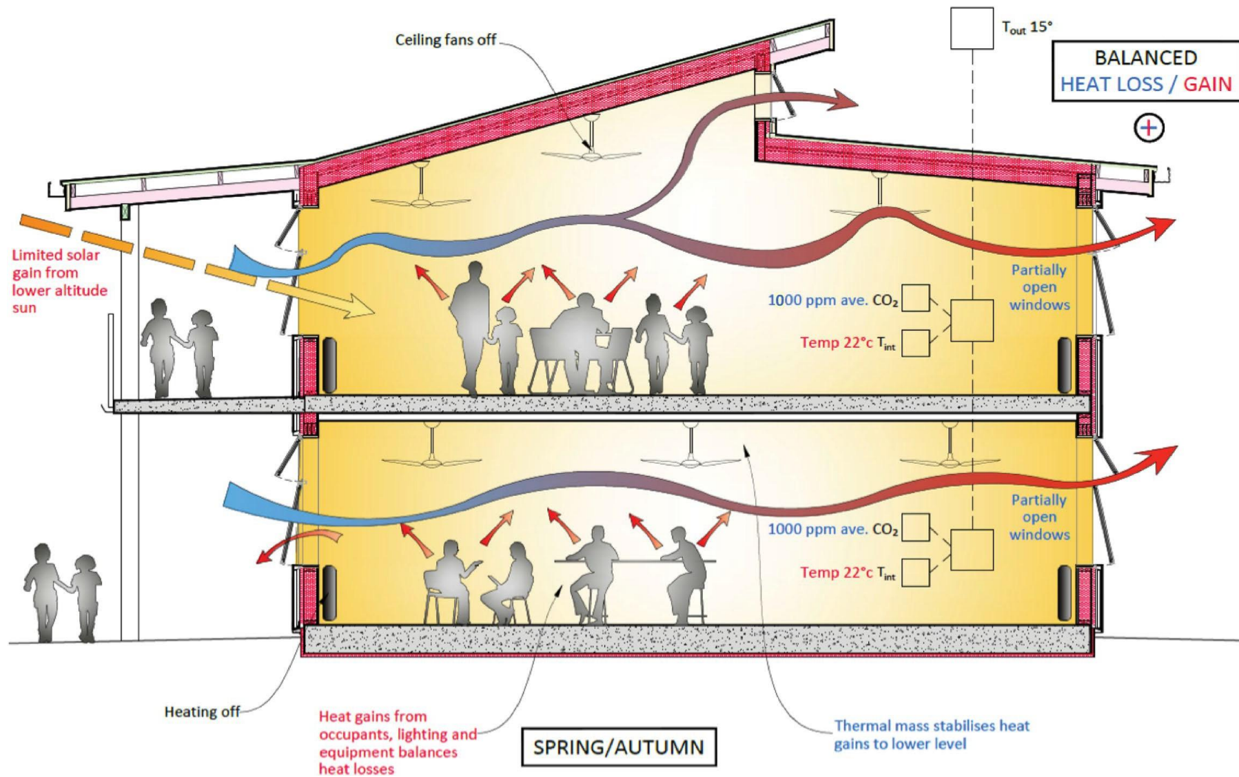
Figure 9: Spring/autumn ventilation modes for typical flexible learning spaces
