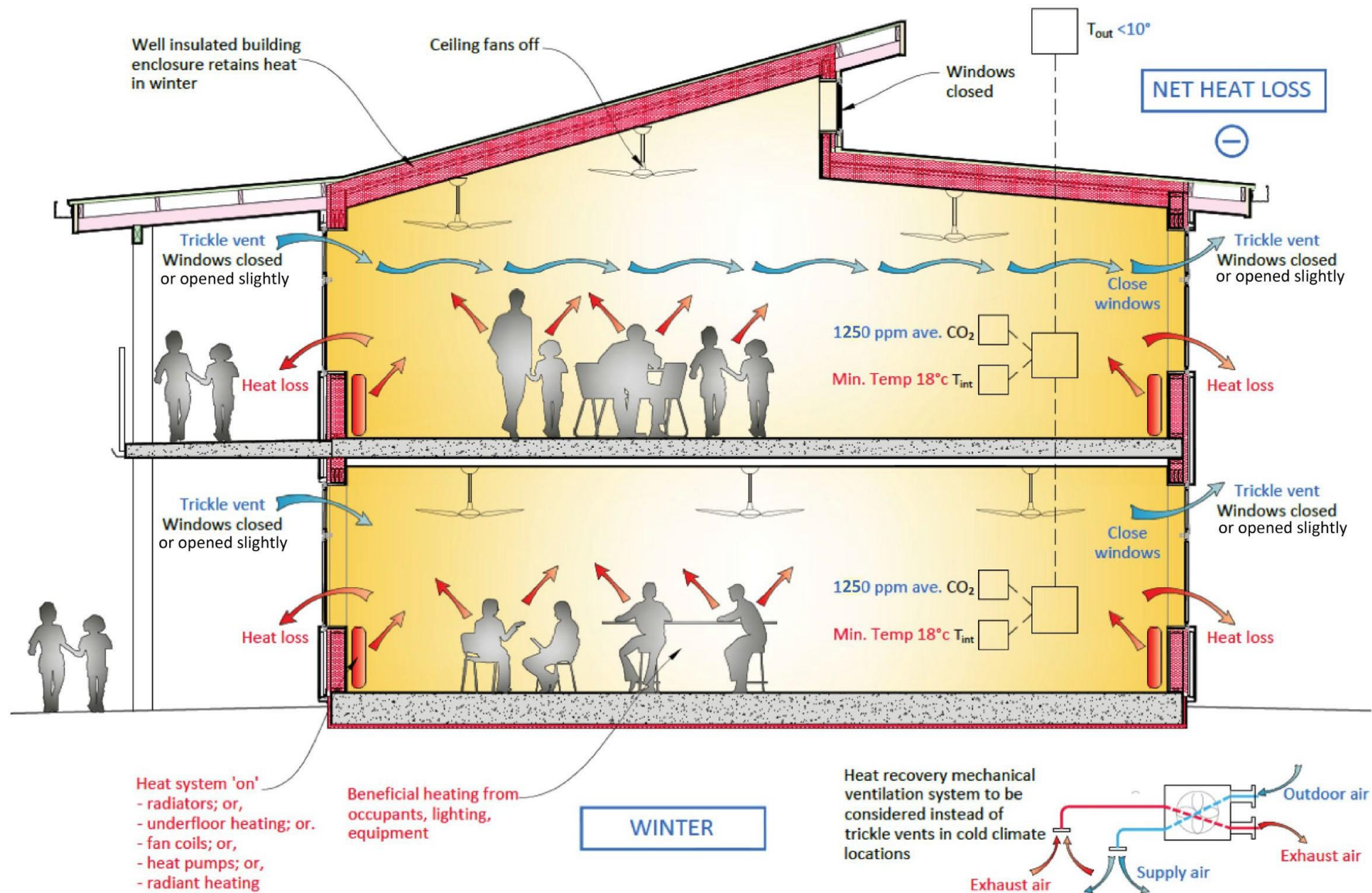
Figure 10: Winter ventilation modes for typical flexible learning spaces
