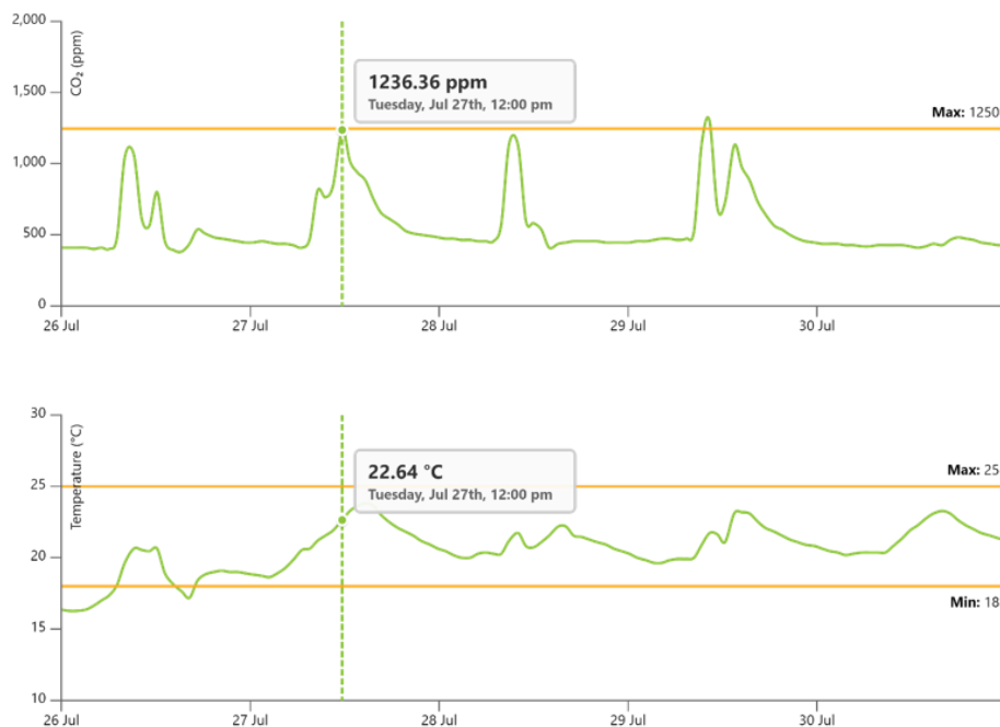
Figure 24: Average CO 2 concentration and temperature levels, in Christchurch District over five winter days, between 12am – 12pm in a primary school learning space
